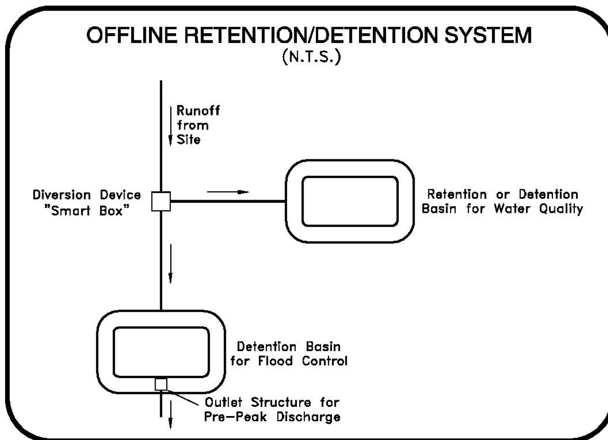
Figure 5-4. Schematic of an Off-Line Retention/Detention System.
